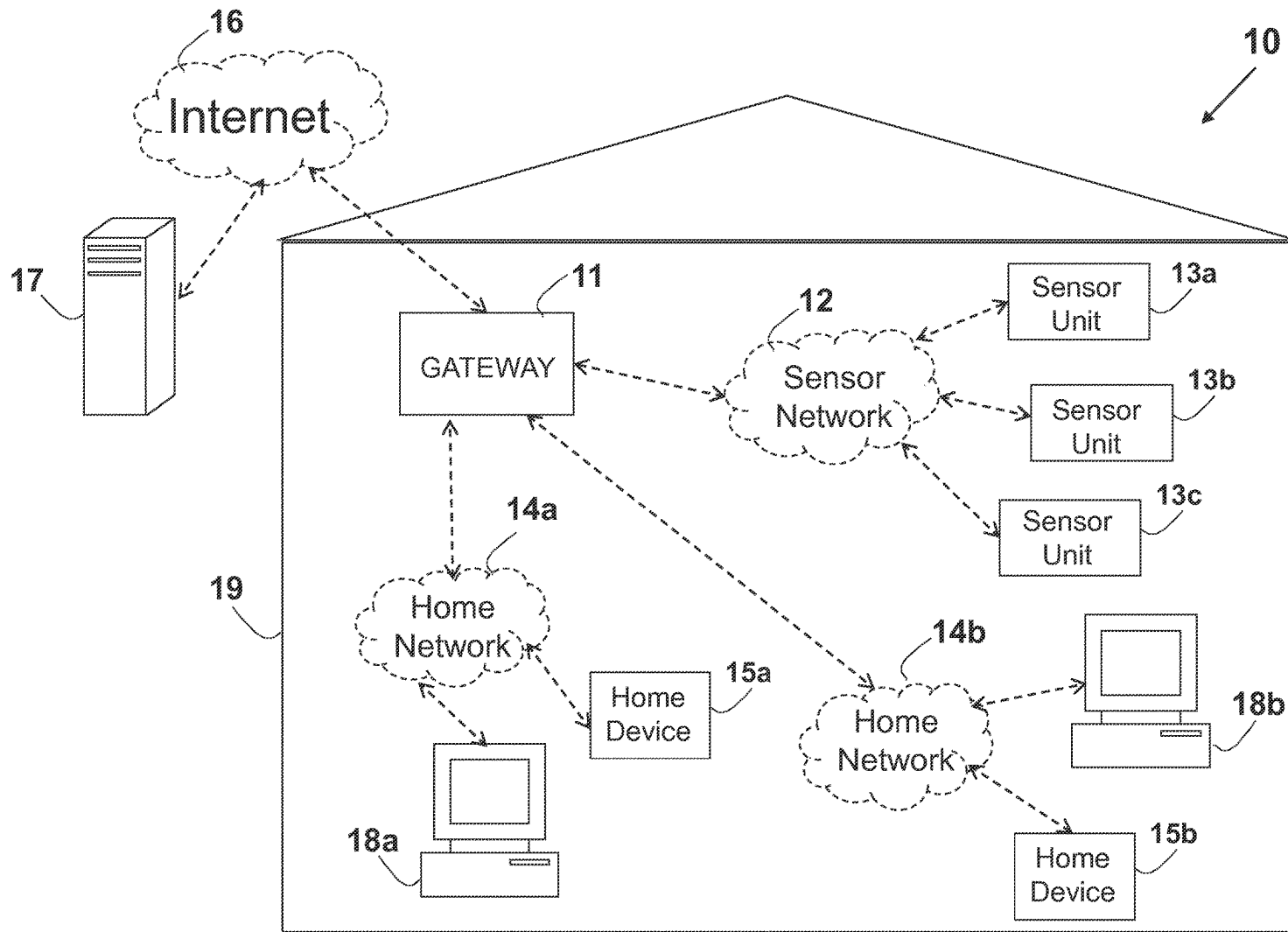
FIG. 1 (Prior Art)
