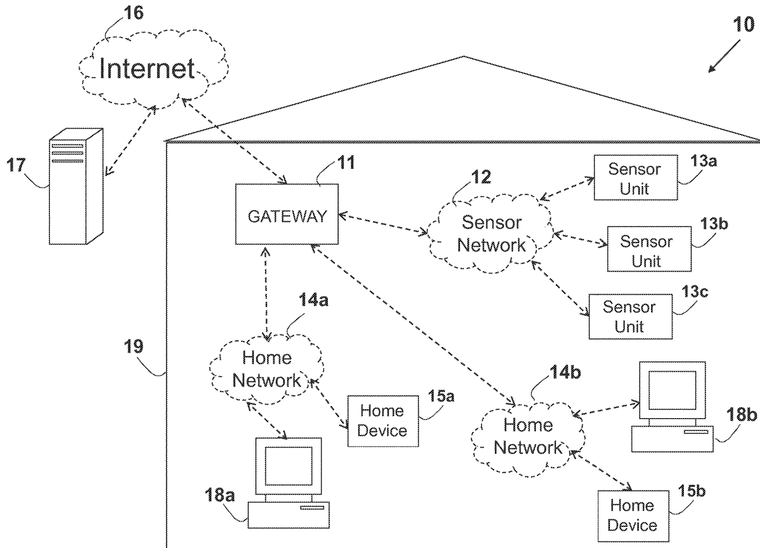
FIG. 1 (Prior Art)
