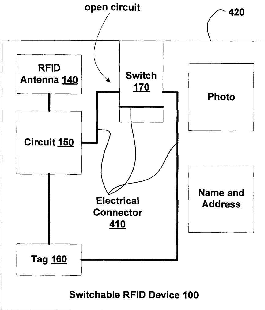
OFF Position FIG. 4A
