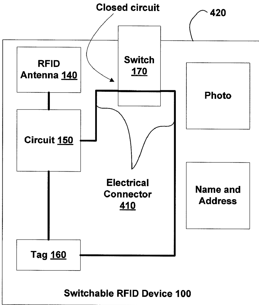
FIG. 4B ON Position
