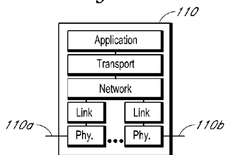
Nomadic Router
