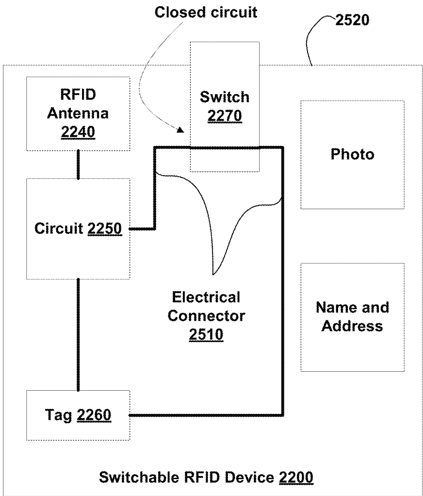
FIG. 25B ON Position
