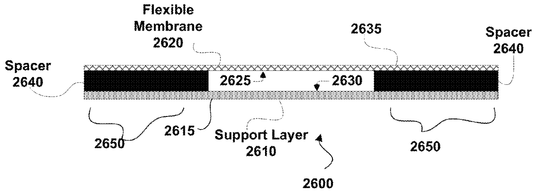
FIG. 26A Membrane Switch (OFF)
